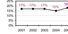
Course Evaluations
