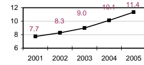
Minority Faculty
