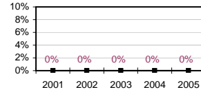
Female Faculty
