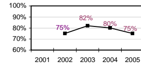
Terminal Degrees
