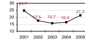
Class Size > 50
